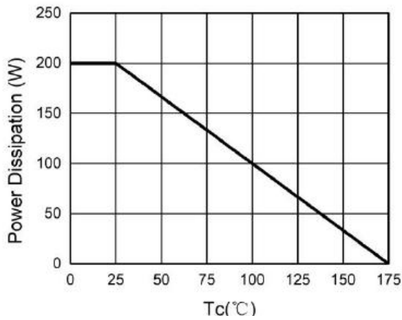
Fig.3 Power Dissipation
