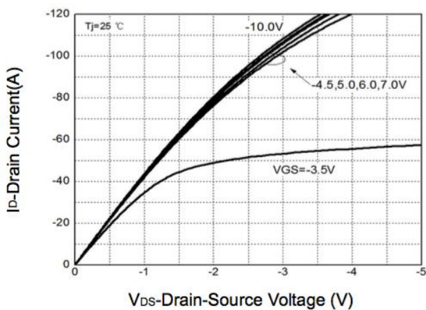
Figure 5: Output Characteristics
